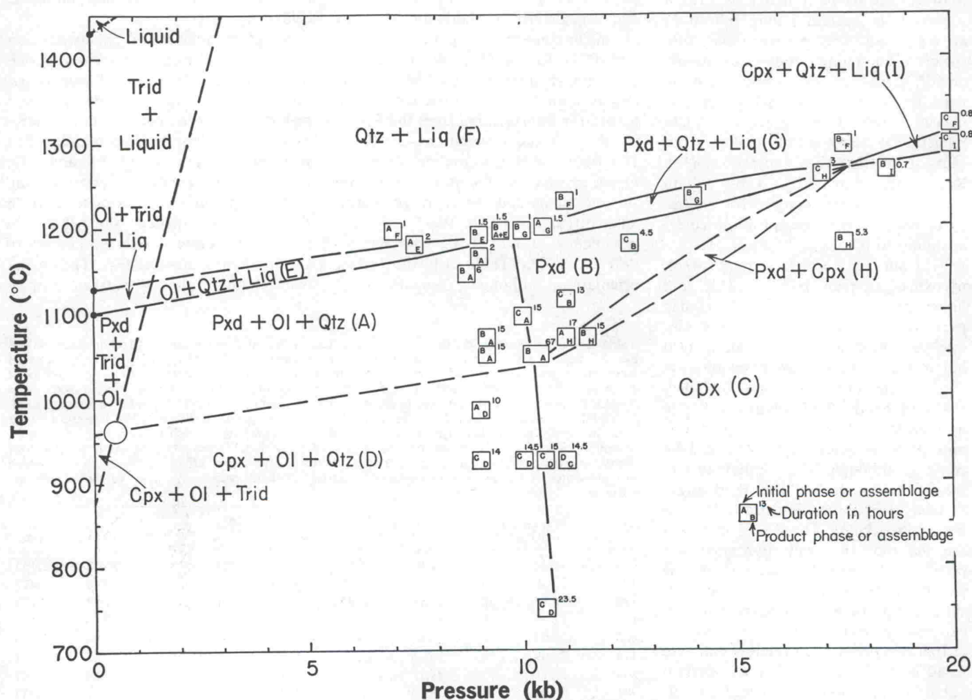
Fig. 1. Pressure-temperature equilibrium diagram for \text{Ca}_{0.15}\text{Fe}_{0.85}\text{SiO}_3 bulk composition, based on experiments with a solid-media, piston-and-cylinder pressure apparatus. Letters within each data symbol indicate for each experiment the initial and product phases or assemblages, and adjacent numerals give the duration in hours. The height of each symbol represents the estimated uncertainty in temperature for each experiment; no correction has been made for the effect of pressure on the platinum versus platinum-90-rhodium-10 thermocouples. The width of each symbol represents the estimated uncertainty in pressure for each experiment (28). Experiments above 925°C were carried out in iron capsules; the loaded capsules were dried overnight under vacuum at 170°C. For experiments at and below 925°C silver capsules were used; to each charge (10 to 15 mg) 1 mg of distilled water and approximately 0.5 mg of pure silica glass were added to saturate the vapor phase during the run (13). These hydrothermal experiments were necessary to obtain suitable rates for the reaction: clinopyroxene \rightarrow Ca-enriched clinopyroxene plus olivine plus \text{SiO}_2 . (Closed circles) Data at a pressure of 1 atm of Bowen et al. (12); (open circle) data from Lindsley and Munoz (13). Liq , liquid containing small amounts of \text{Fe}_2\text{O}_3 ; Qtz , quartz; Trid , tridymite; Ol , olivine rich in \text{Fe}_2\text{SiO}_4 ; Cpx , clinopyroxene; Pxd , pyroxenoid. The iron content of pyroxenoid and clinopyroxene that coexist with olivine and a silica phase in this diagram must always be less than \text{Ca}_{0.15}\text{Fe}_{0.85}\text{SiO}_3 and will decrease with decreasing pressure. The structures of these iron-depleted pyroxenoids are unknown; they may be of the Fünferketten or Dreierketten type, or both.
